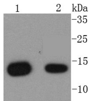
Fig. 1. Western blot analysis of beta 2 Microglobulin on different lysates using anti-beta 2 Microglobulin antibody at 1/1,000 dilution. Positive control: Lane 1: Raji; Lane 2: U937
